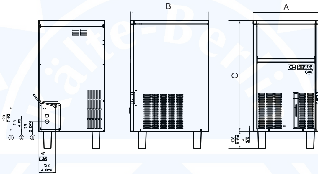
SDN 35 - 45 - 65
