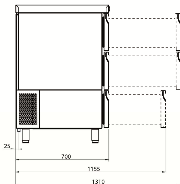
Model HDCF13E (type HDCF13E)
