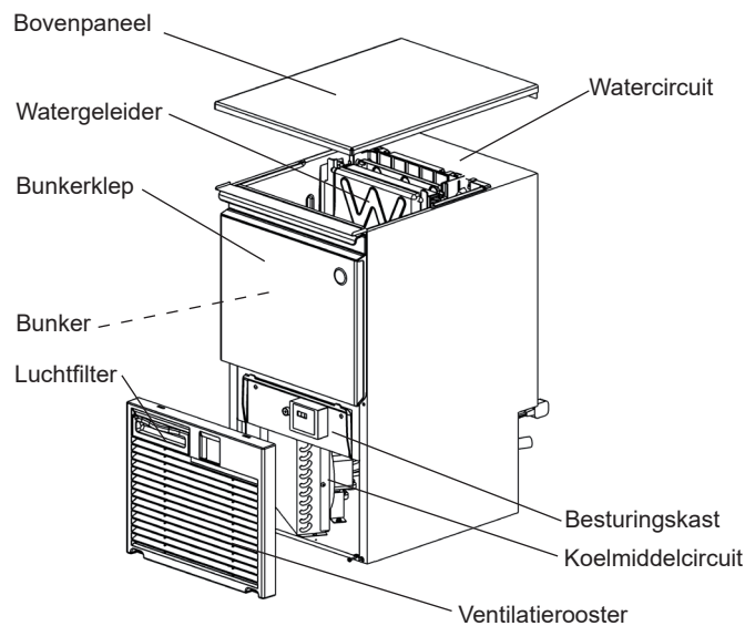
KM-40/60/80C-HC
