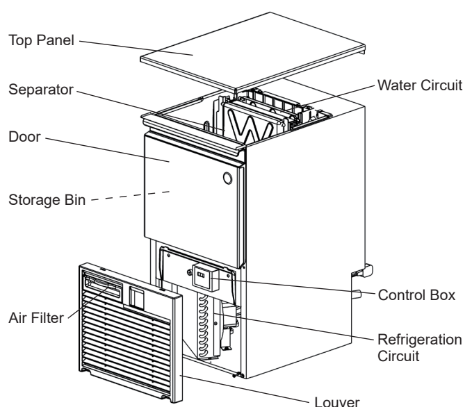
KM-40/60/80C-HC
