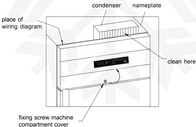
Picture 3: Cleaning of condenser
