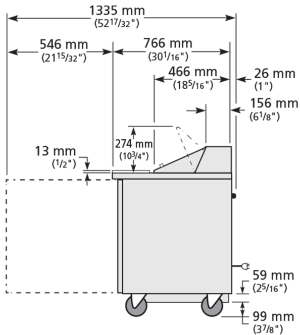
RIGHT VIEW
