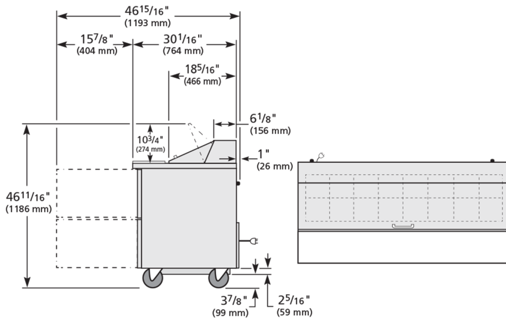
RIGHT VIEW
