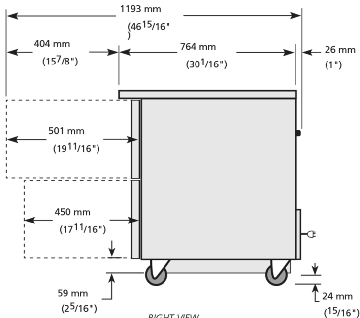
RIGHT VIEW
