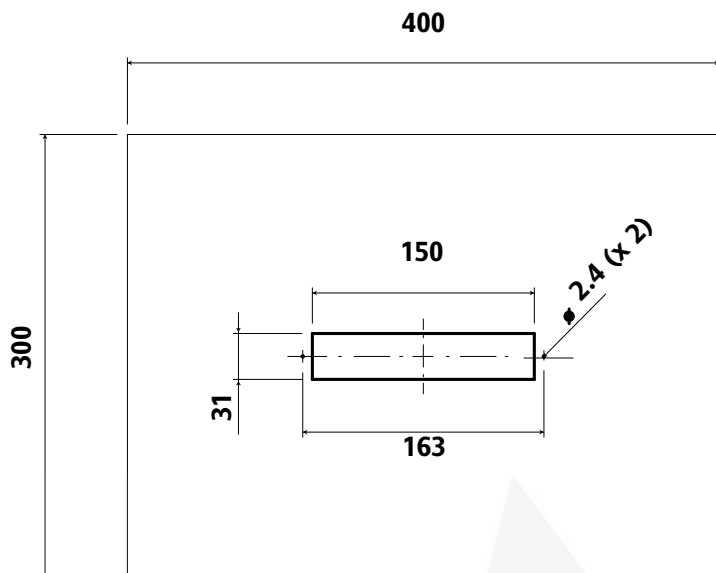
(A) PANEL THICKNESS 0.5-1-1.5-2-2.5-3 mm
