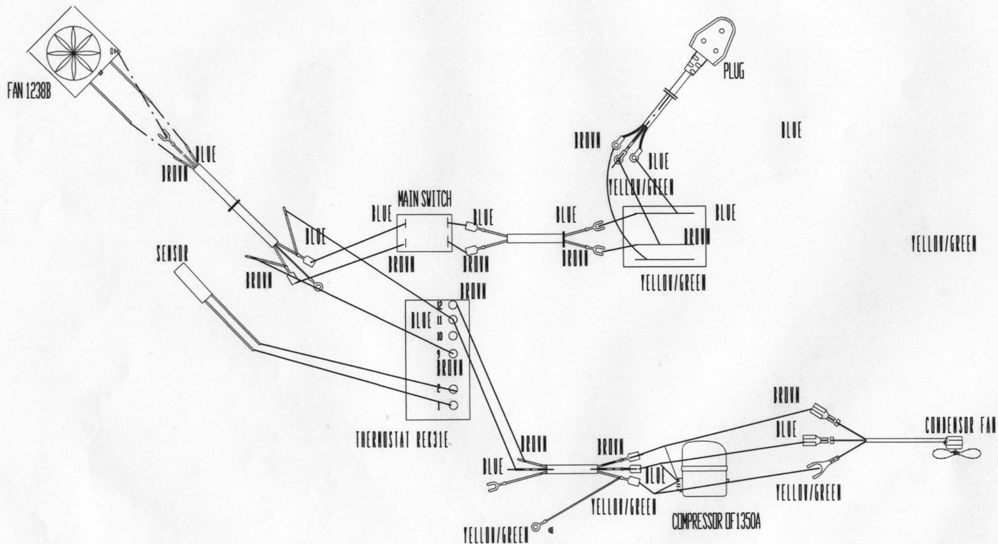
WIRING DIAGRAM OF S900 PS900 S900. TOP. S/S
