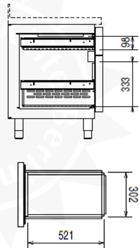
1x1/2+2x2/3 Schubladen
