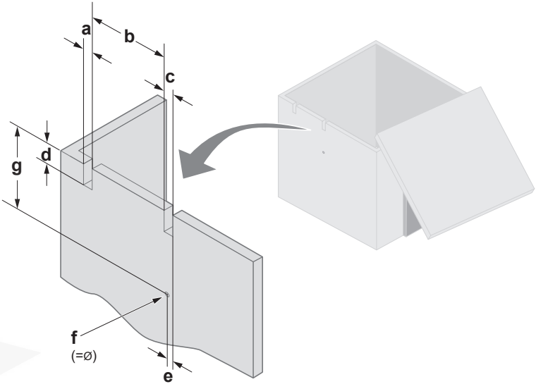
Sattelmontage
